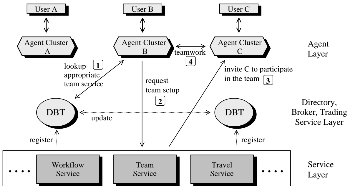
Figure 1: System Architecture
