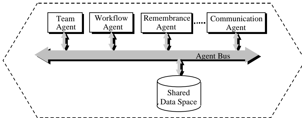
Figure 2: Agent Cluster
