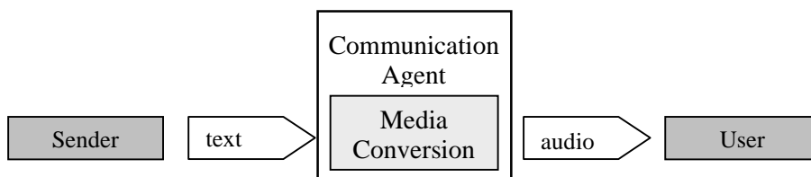
Figure 3: Media Conversion
